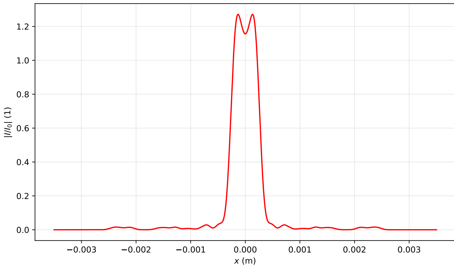
Intensity profile I(x, y = 0, z = 3.105)/I_0 , P_{in}=3.0P_{cr} , artificial time
